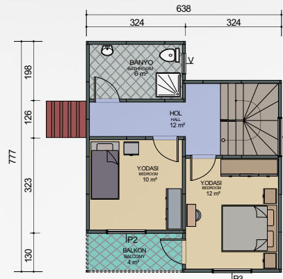
1. KAT PLANI FIRST FLOOR PLAN 41 m² + 4 m² = 45 m²
