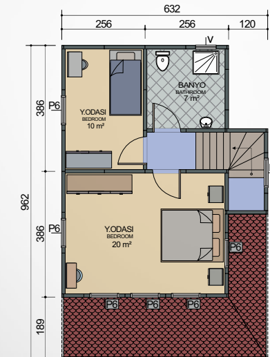
1. KAT PLANI FIRST FLOOR PLAN
