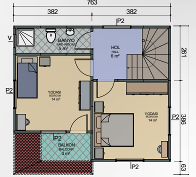
1. KAT PLANI FIRST FLOOR PLAN 45 m² + 3 m² = 48 m²
