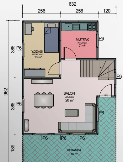
ZEMİN KAT PLANI GROUND FLOOR PLAN
