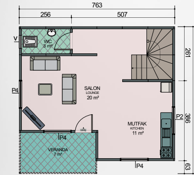
ZEMİN KAT PLANI GROUND FLOOR PLAN 45 m² + 7 m² = 52 m²
