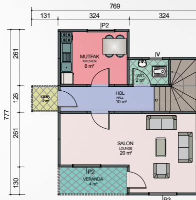
ZEMİN KAT PLANI GROUND FLOOR PLAN 41 m² + 6 m² = 47 m²
