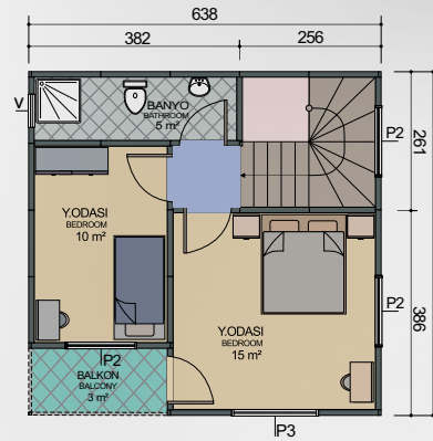
1. KAT PLANI FIRST FLOOR PLAN 37 m² + 3 m² = 40 m²
