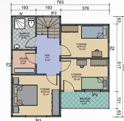
1. KAT PLANI FIRST FLOOR PLAN 49 m² + 5 m² = 54 m²
