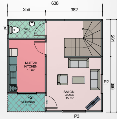
ZEMİN KAT PLANI GROUND FLOOR PLAN 37 m² + 3 m² = 40 m²
